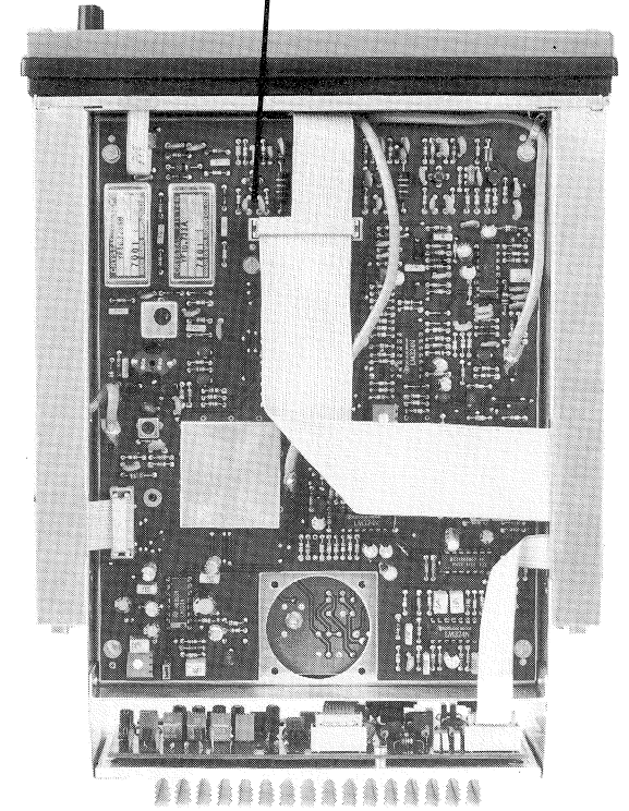
Receiver Unit (Module 1)
